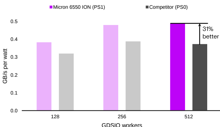
Figure 7: 16KB transfer power efficiency (GB/s per watt, higher is better)
