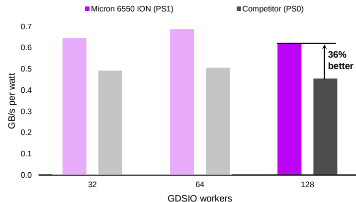
Figure 9: 128KB transfer power efficiency (GB/s per watt, higher is better)
