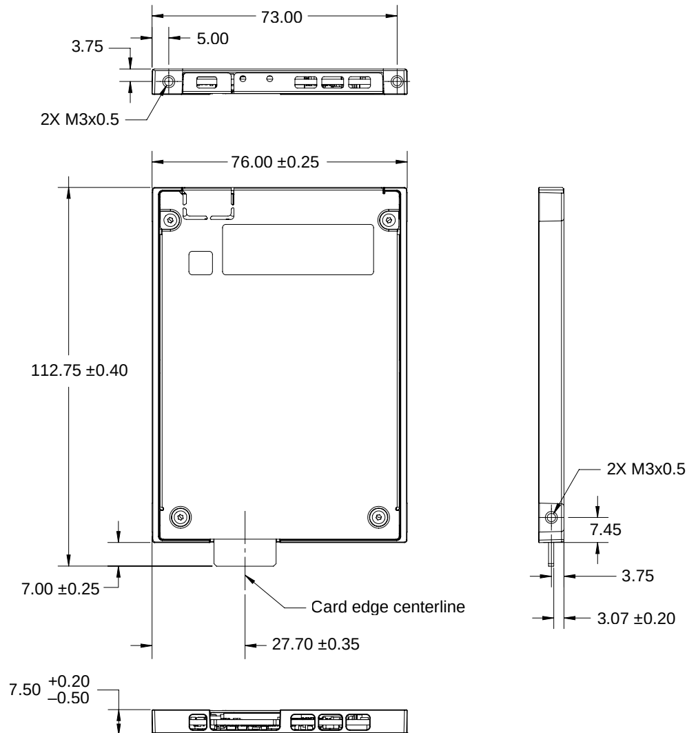
Figure 5: E3.S 1T 7.5mm Nominal Dimensions
