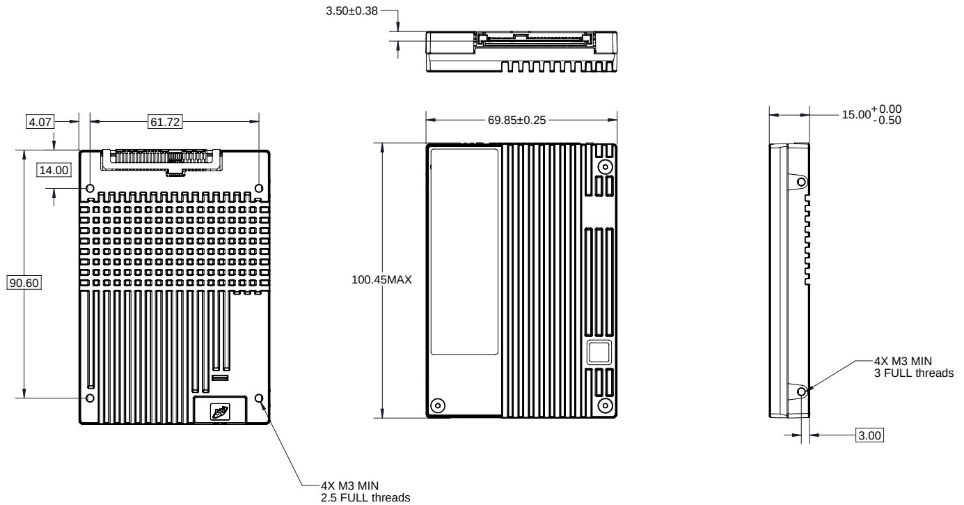
Figure 2: U.2 30T7 15mm Nominal Dimensions
