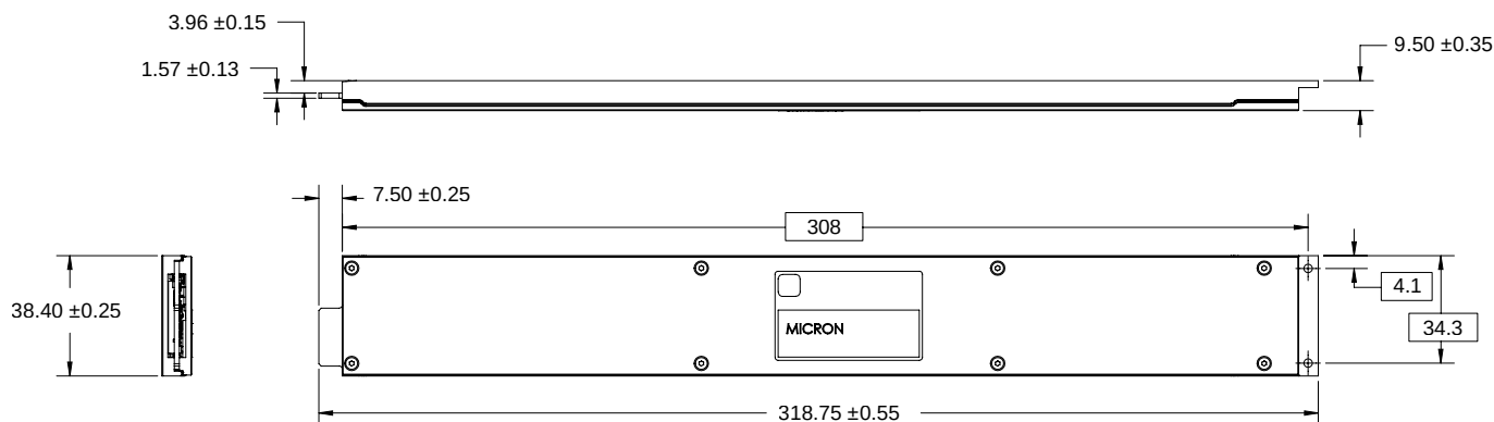
Figure 4: E1.L 9.5mm Nominal Dimensions
