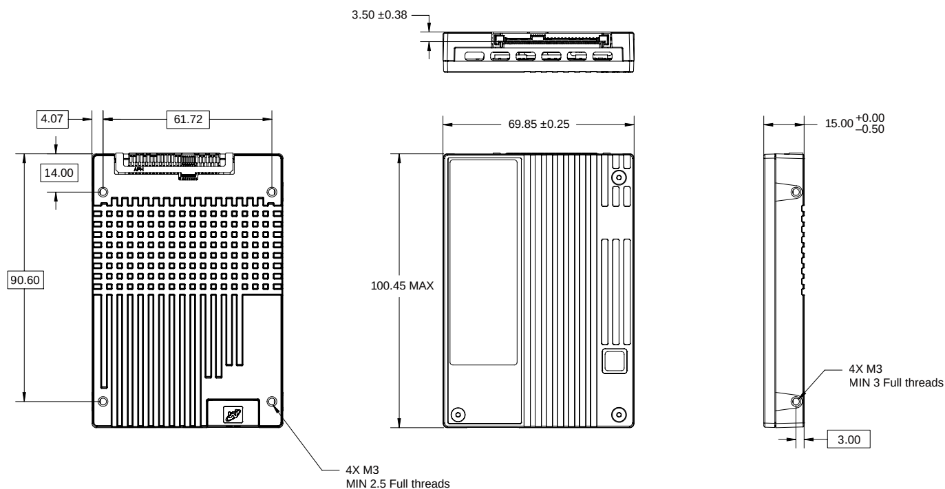
Figure 3: U.2 61T4 15mm Nominal Dimensions
