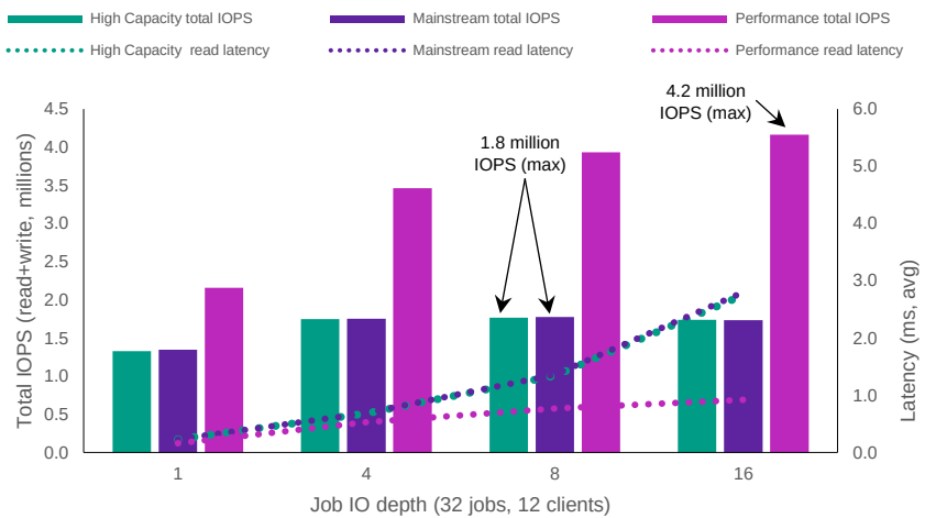
Figure 6: 4KB mixed 100% random 50% read, 50% write
