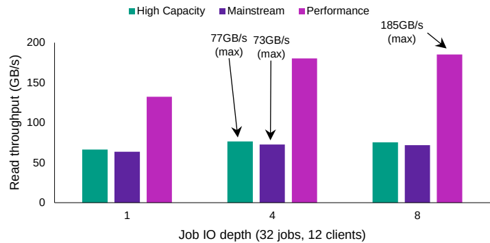
Figure 8: 128KB 100% sequential 100% read
