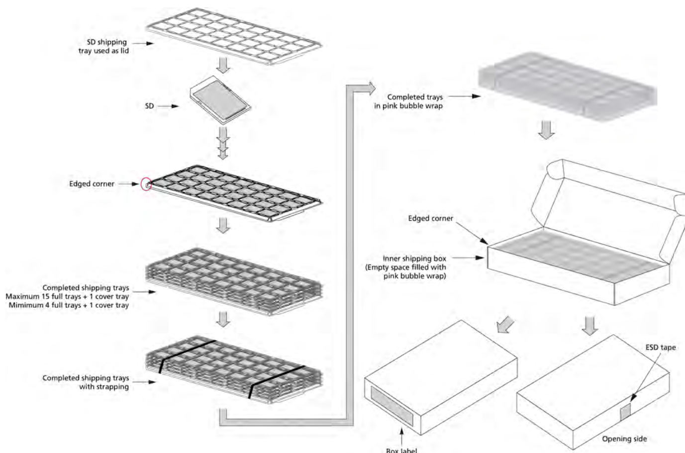
Figure 13: SD Packaging
