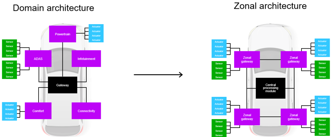
Figure 8: Domain versus zonal architecture
