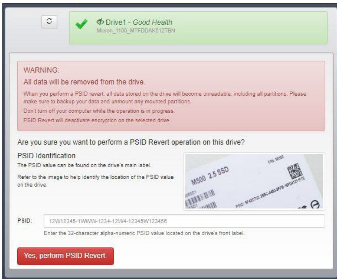
Figure 19: PSID Revert
