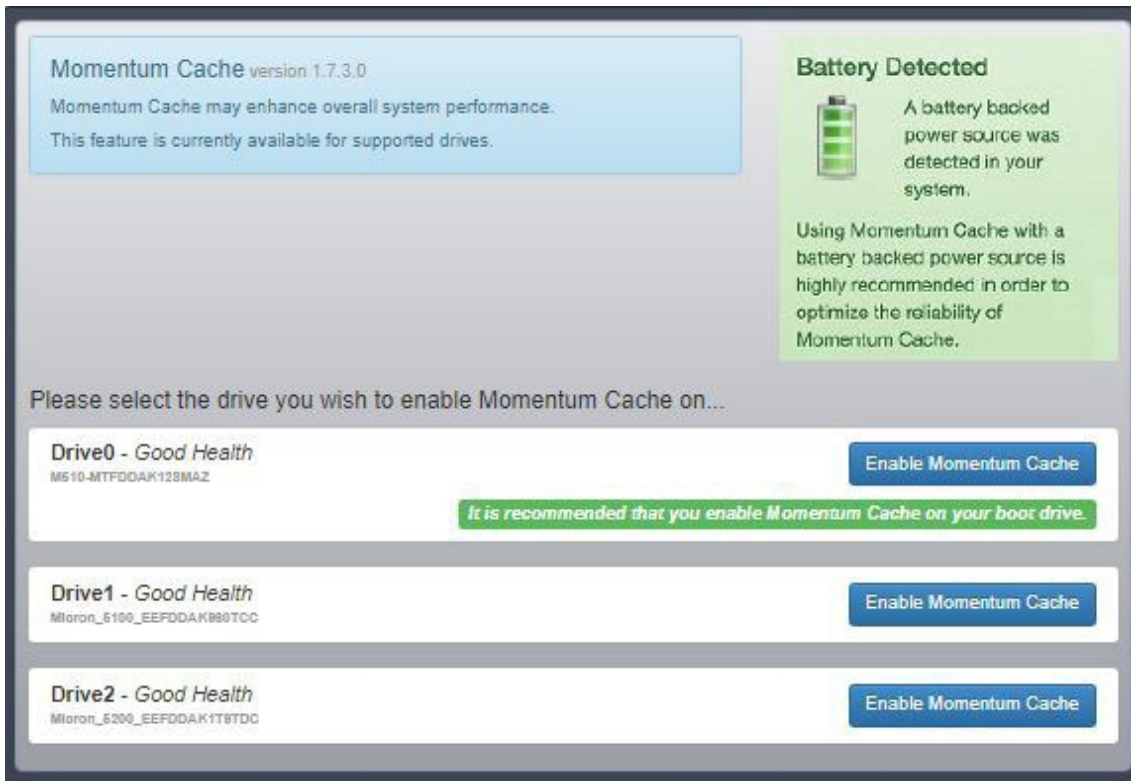
Figure 20: Momentum Cache
