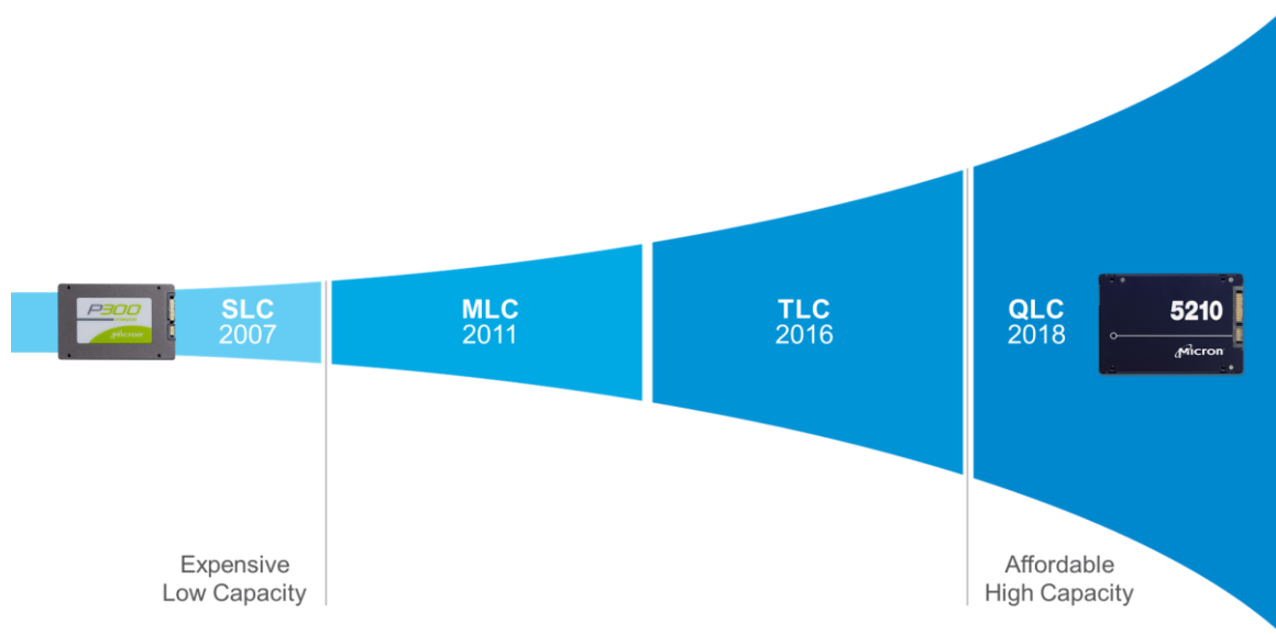
Figure 3: SSD Trends
