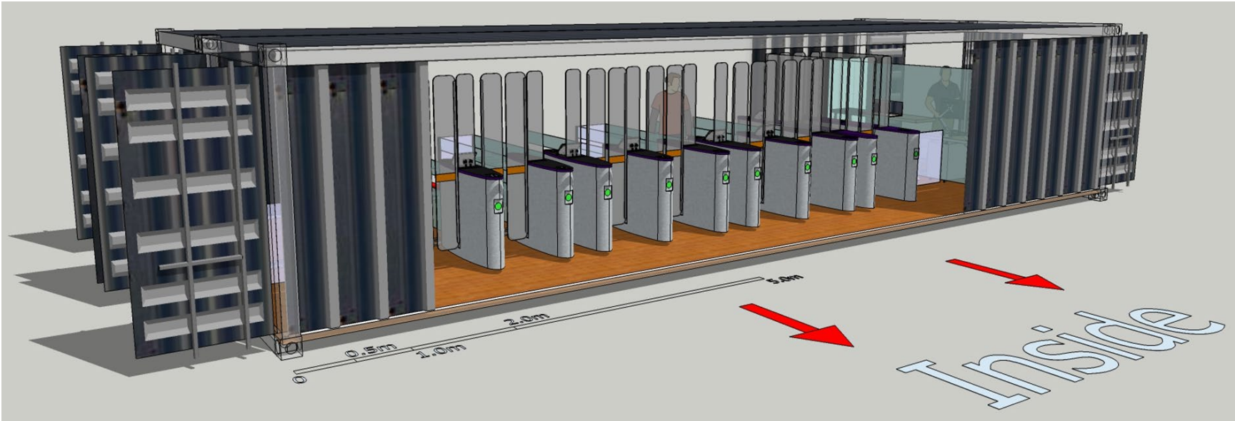
Figure 9 Containerized Access Control System
